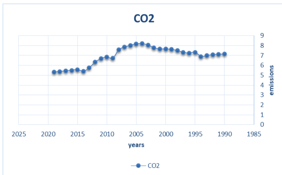
Figure.(2) CO2.emissions.(metric.tons.per.capita)
