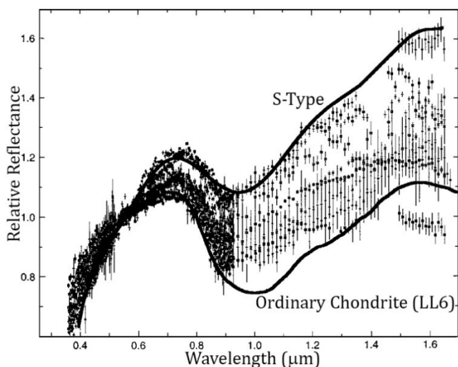
Fig. 2. S- to Q-class transition within the NEAs population. Fig. 2 adopted from Binzel et al. (2001) .
