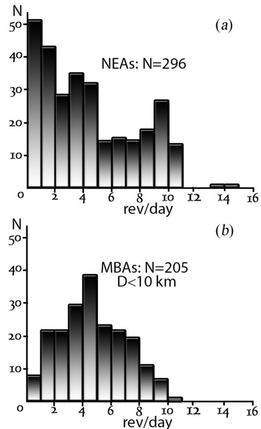
Fig. 1. Distribution of rotational rates as a function of speed of rotation: a- rotation rates of 296 NEAs; b- rotation rates of 205 MBAs with D < 10 km
