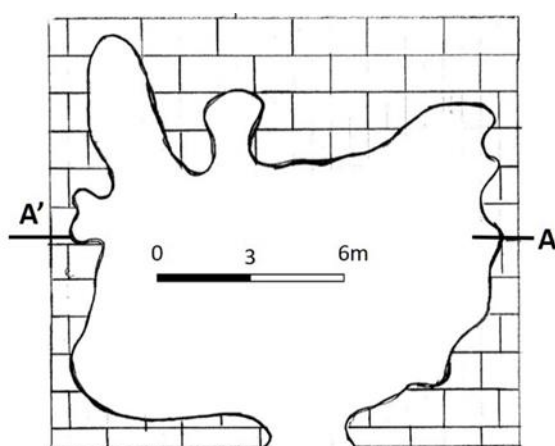
Fig. 26. Plane view of Wadi Belgares Cave
