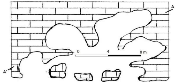
Fig. 23. Plan view of Wadi Asoukunyah Cave
