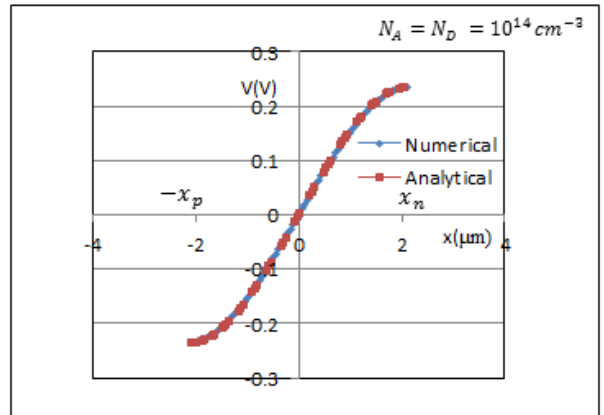
Fig. 5. Electrostatic potential for fixed charge density of impurities [ N_A , N_D ] within depletion layer
