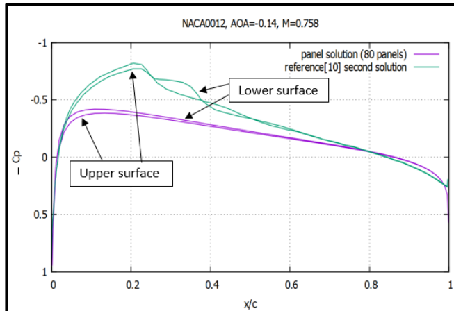
Fig. 20. Comparison of Panel Solution with Second Solution Given in (Sengupta et al., 2013).
