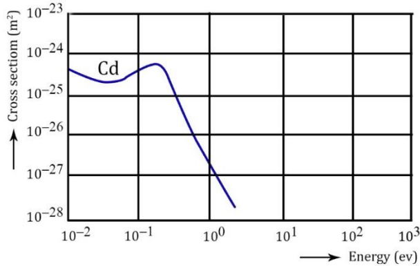
Fig. 1. Thermal neutrons activation cross-section of cadmium
