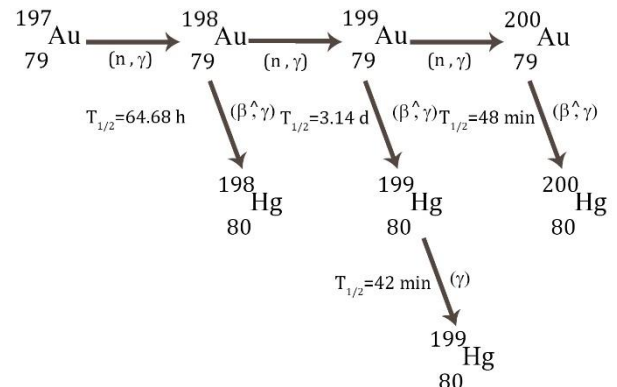
Scheme 2. Au reaction with neutron
