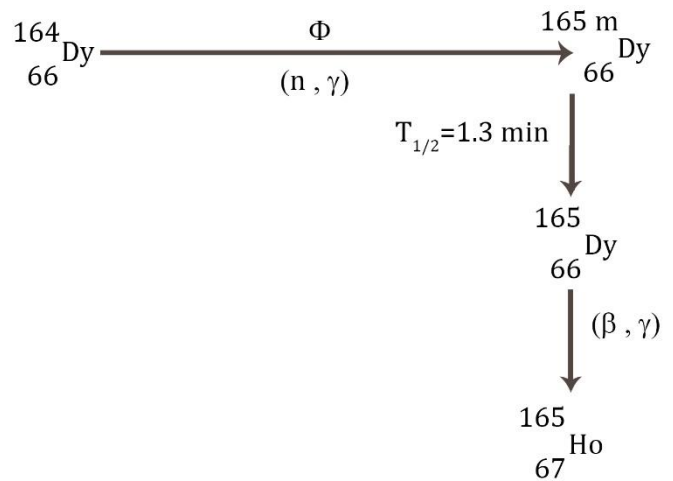
Scheme. 1. Dy reaction with neutron
