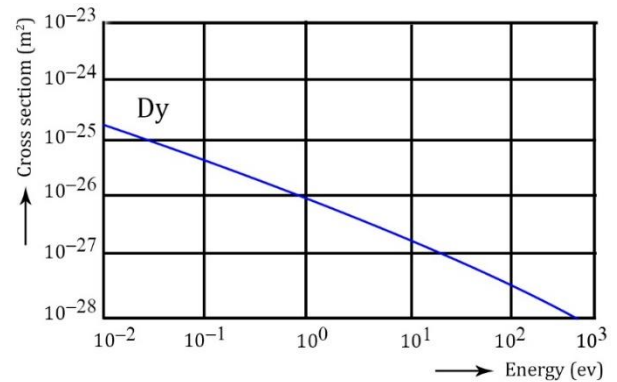
Fig. 2: Thermal neutrons activation cross-section of Dy
