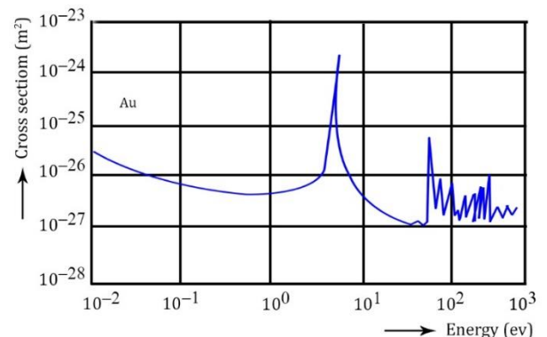
Fig. 3. Thermal neutrons activation cross-section of Au
