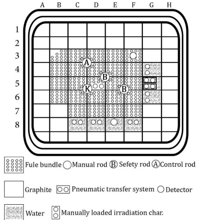
Fig. 4: BTU research reactor core (top view)
