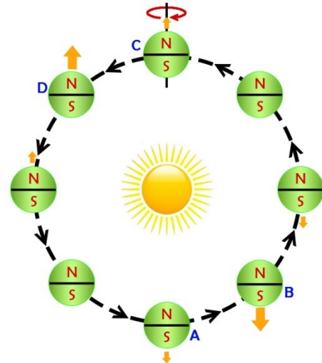
Fig.4. The seasonal, Yarkovsky effect is caused by the fact that the seasonal heating of northern and southern hemispheres of solar system bodies peaks at a point somewhat after the solstices. This seasonal Yarkovsky effect results the thermal force lying along the spin axis.
