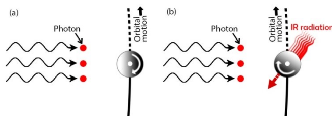
Fig. 1. a- Photons are incident on an asteroid spinning in prograde sense of rotation with spin axis perpendicular to the orbital plane. b- Radiation is emitted typically in the infrared part (IR) of the spectrum, unless the meteoroid is very close to the Sun. A case of asteroid slowing down.
