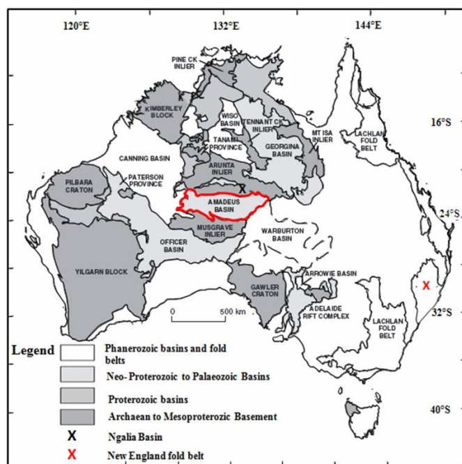
Fig. 1. The Australian intracratonic sedimentary basins that comprise the Amadeus basin (red outline), Georgina basin, Officer basin and Ngalia basin (modified after Maidment et al. , 2007).
