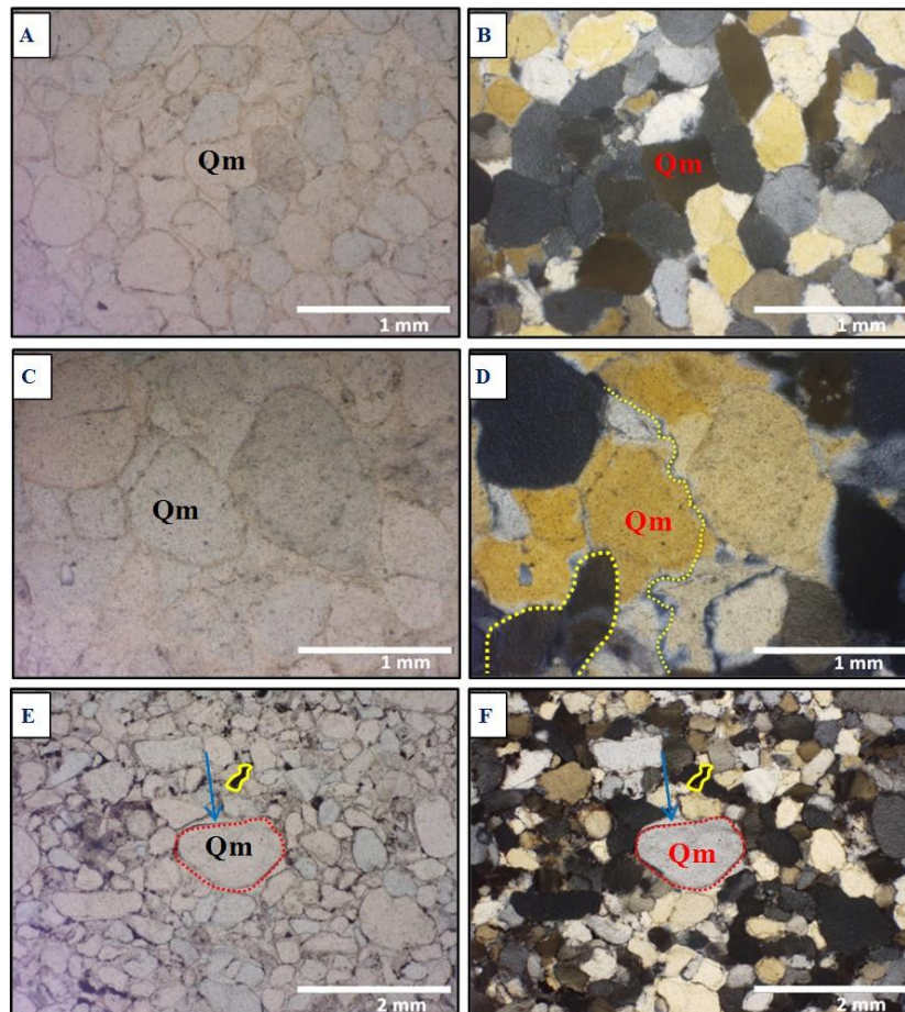
Fig. 6. Photomicrographs (A) and (B) Well rounded, well sorted and well compacted monocrystalline quartz grains (unit 6); (C) and (D) Sutured grain contact. Note all grains are well compacted and there is dissolution due to pressure-solution (unit 4) and (E) and (F) Quartz overgrowth cement (authigenic cement) (unit 1).
