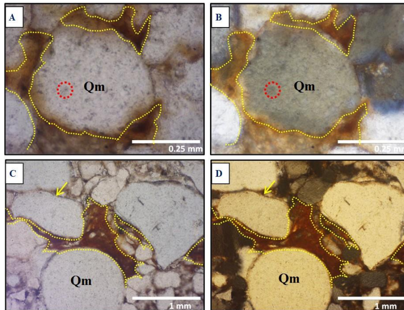
Fig. 7. Photomicrographs (A) and (B) Monocrystalline quartz grains with non-undulatory extinction surrounded by hematite cement (authigenic cement). These quartz grains contains fluid inclusions (unit 1) and (C) and (D) Oversized pore space around well rounded quartz grains due to the dissolution of quartz overgrowth cement, and then filled by hematite cement between quartz grain (unit 1).
