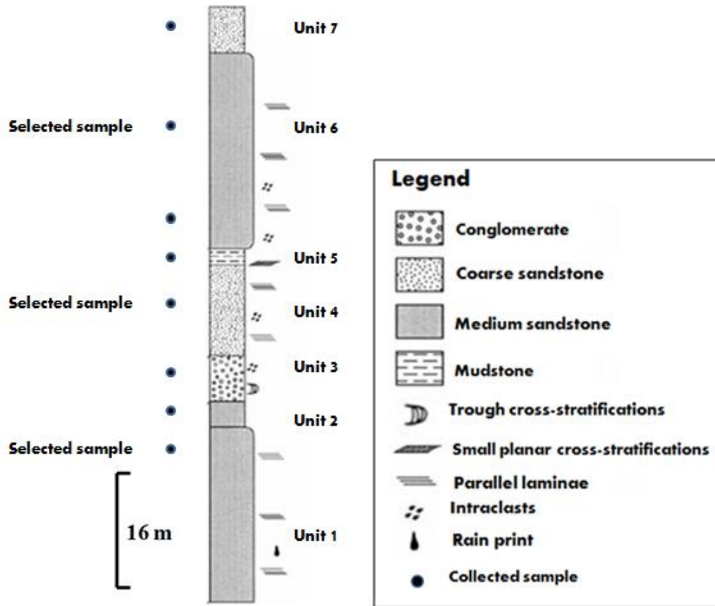
Fig. 4. Sedimentological log of the Heavitree Quartzite shows seven lithofacies.
