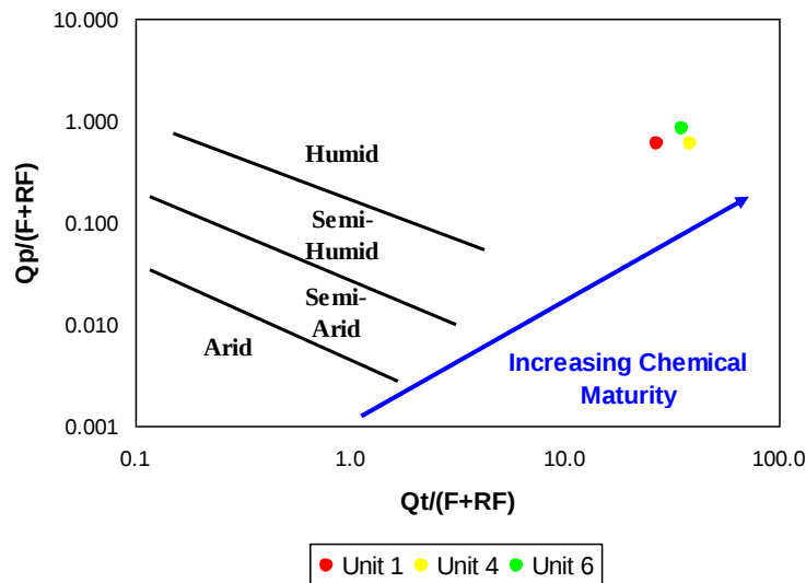
Fig. 11. Climatic discrimination diagram of major components for the Heavitree Quartzite (fields after Suttner and Dutta, 1986).
