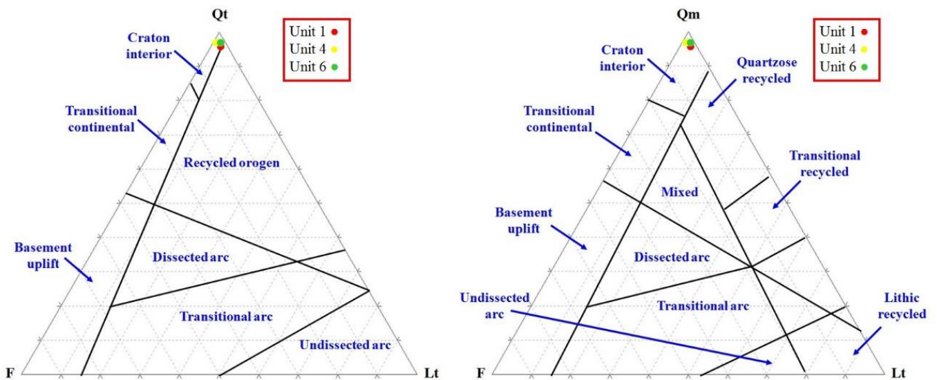
Fig. 9. Tectonic discrimination diagrams of major components for the Heavtree Quartzite (fields after Dickinson et al., 1983).
