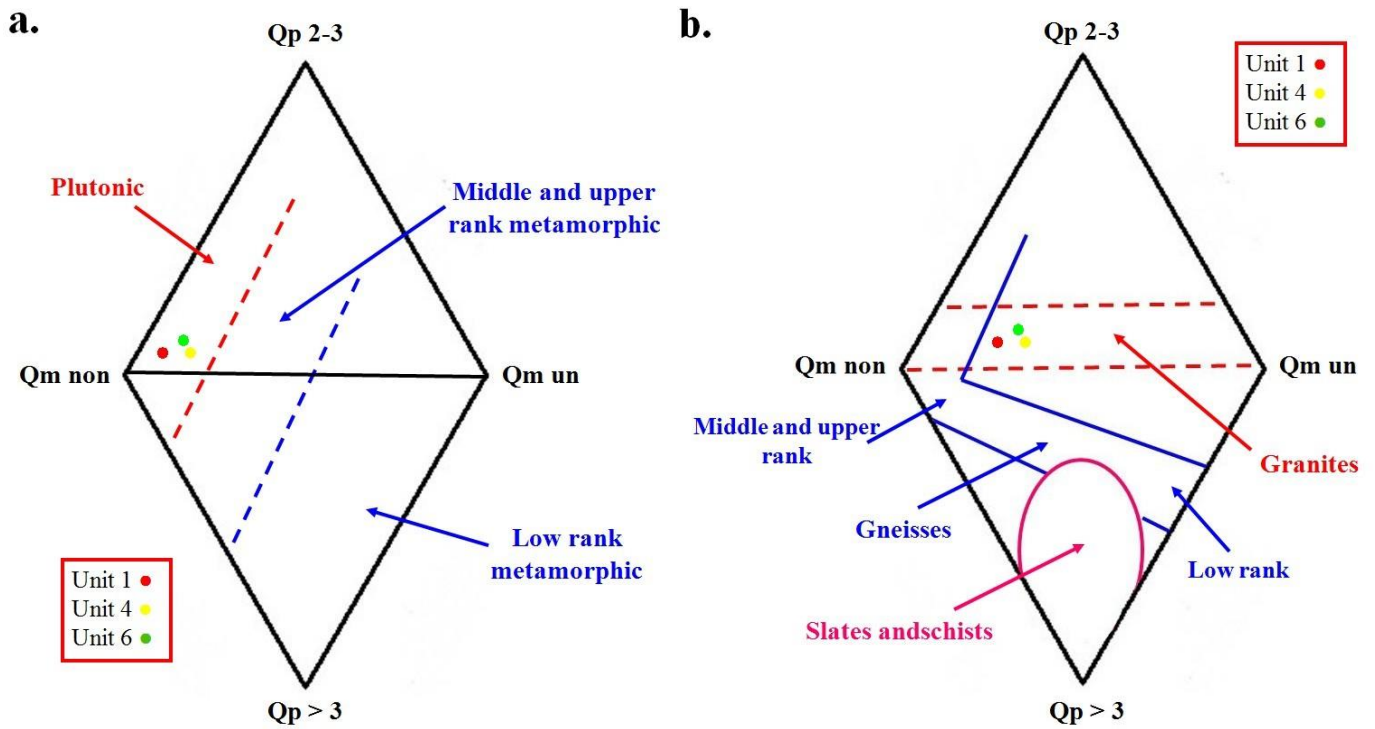
Fig. 8. Varietal quartz diamond plot currently used to discriminate sandstones sourced by different types of crystalline rocks, based on the extinction pattern and polycrystallinity of quartz grains. Qm non = low-undulosity monocrystalline quartz grains; Qm un = high-undulosity monocrystalline quartz grains; Qp2-3 = coarse-grained polycrystalline quartz grains; Qp > 3 = fine-grained polycrystalline quartz grains (fields after Basu et al., (1975) and Tortosa et al., (1991) (diagrams a and b, respectively).
