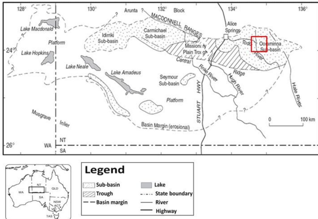
Fig. 2. Major morphological features of the Amadeus basin, the study area in red square (modified after Lindsay and Korsch, 1991).
