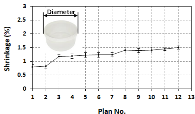
Fig. 5. Measurements of shrinkage at diameter position
