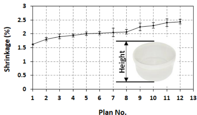
Fig. 6. Measurements of shrinkage at a height position
