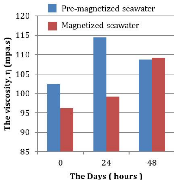
Fig. 9. The viscosity of seawater concentrations during days at 80%.
