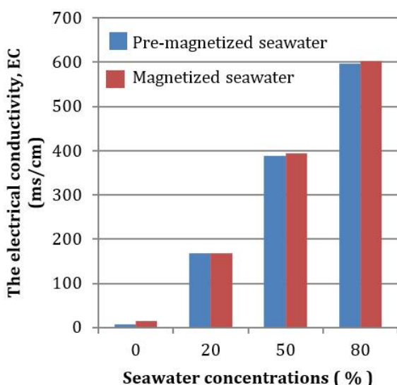
Fig. 6. The electrical conductivity of seawater concentration (Pre-magnetized & Magnetized) at 21.3^\circ\text{C} .
