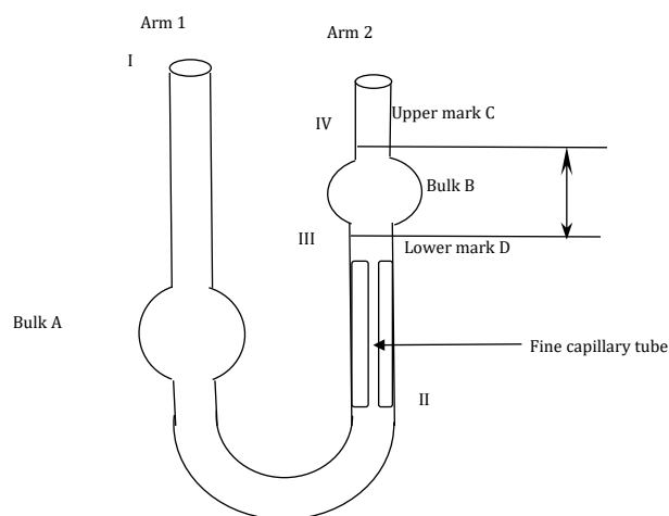
Fig. 3. The tool of measuring the viscosity.
