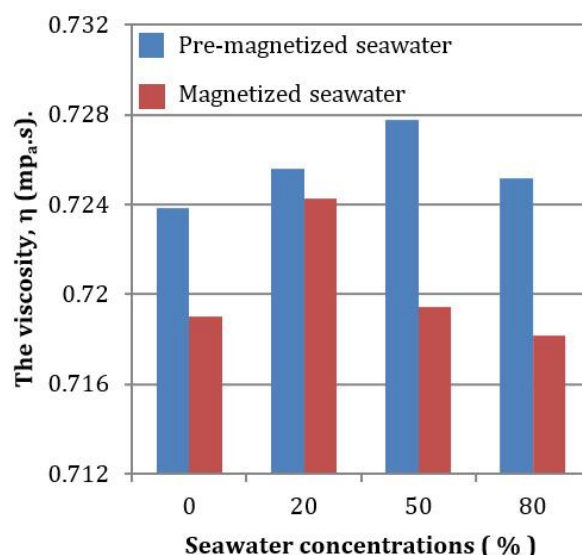
Fig. 8. The viscosity of seawater concentrations (Pre-magnetized & Magnetized) at 21.3^\circ\text{C} .
