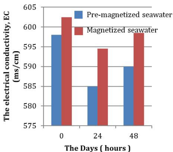
Fig. 7. The electrical conductivity of seawater concentrations during days at of 80%.
