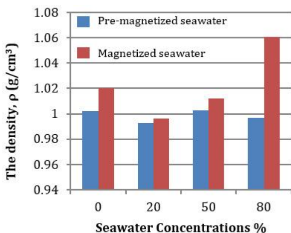
Fig. 4. The density of sea water Concentrations (Magnetized & Pre-magnetized) at 21.3 °C.
