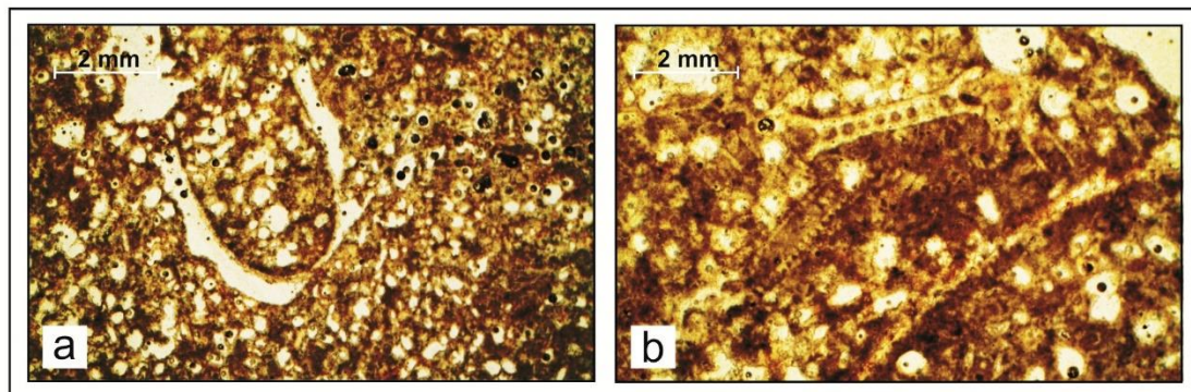
Fig. 6. Photomicrographs showing mostly mud-supported wackestone-packstone texture with abundant micrite-clasts (tiny brown pellets). Both microfacies are representing the typical lithology of the Upper Paleocene Bú Rá's Member, lower member of the Shurfah Formation, at Wadi Marzuq section. The sediments are completely made-up of tiny circular (white circles) including U-shape (at the middle) Dasycladacean and Codiacean green algae (a). Longitudinal sections (yellowish-brown) with a characteristic internal structure of Dasycladacean and Codiacean green algae are also present (b).
