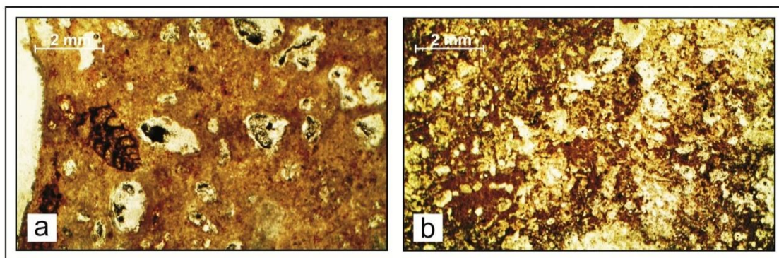
Fig. 9. Photomicrograph showing mostly mud-supported wackestone with undifferentiated shell fragments of pelecypods (white colors) and biserial (left side) small benthic foraminifera (a). Photomicrograph showing gypsiferous dolomitic marly limestone enriched mostly by shell fragments of pelecypods (white colors) (b). Both microfacies are belonging to the Khayir Member, lower member of the Bishimah Formation (Lower Eocene), at the Wadi Marzuq section.
