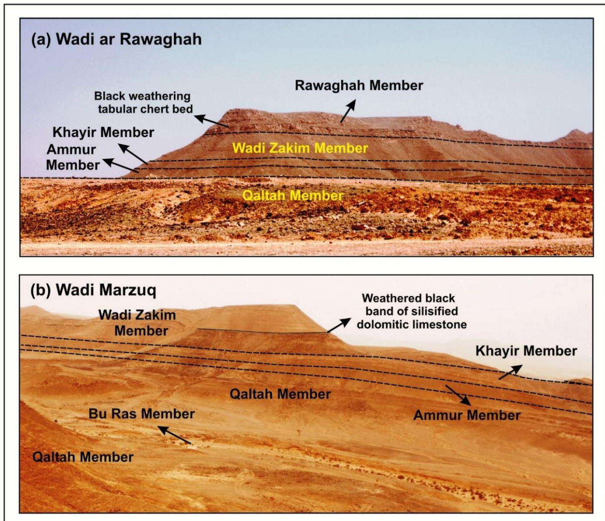
Fig. 3. Views of the studied outcrops showing the studied rock units at Wadi ar Rawaghah (a), and Wadi Marzuq (b).
