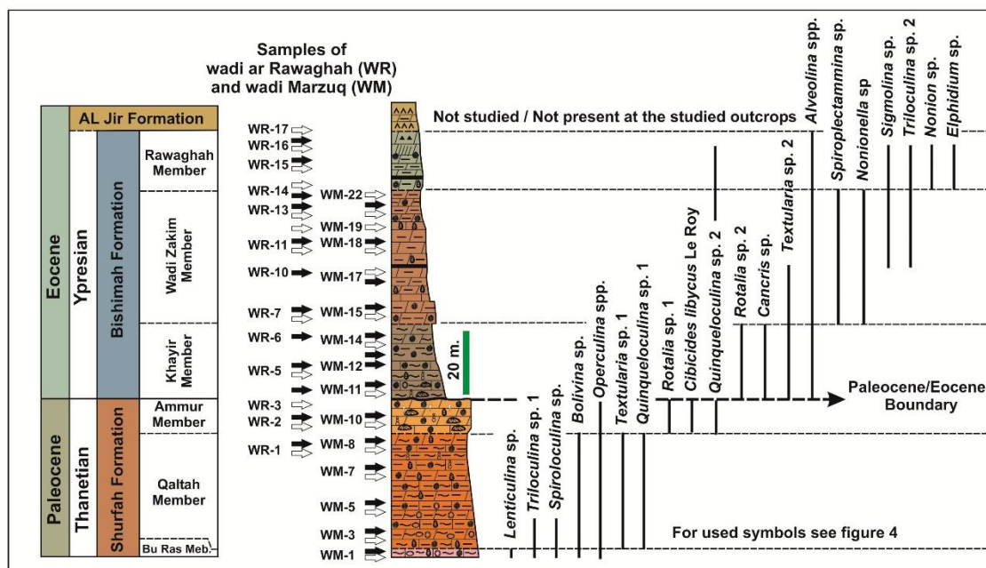
Fig. 12. Composite stratigraphic occurrences chart of the studied foraminifera in the study area.
