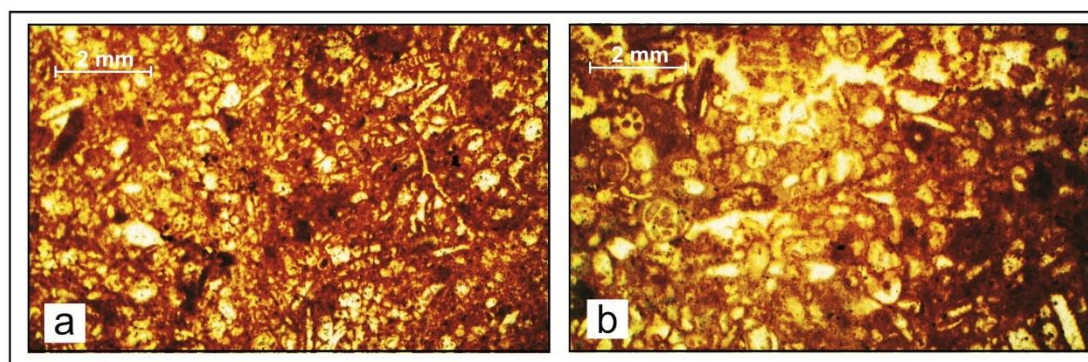
Fig. 8. Photomicrographs showing mostly bioclastic and mud-supported wackestone-packstone. Both microfacies are belonging to the Ammúr Member, the upper member of the Shurfah Formation (Upper Paleocene). Tiny circular (white colors) and longitudinal sections (tiny needle-shaped) of Dasycladacean and Codiacean green algae and unrecognized small-sized shallow benthic foraminifera are quite common in the lower levels at Wadi Marzuq section (a). Shallow small benthic foraminifera (left side); other shell fragments (dispersed) and bladed crystals of calcite (dispersed) are major constituents to the study sediments in the upper levels at Wadi ar Rawaghah section (b).
