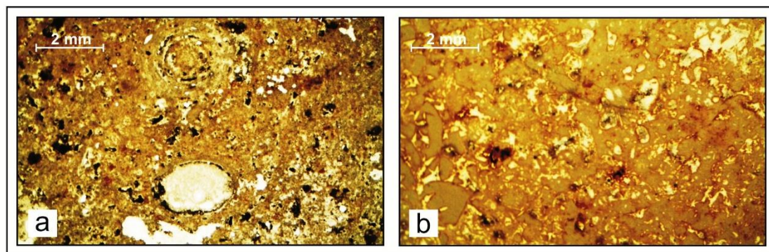
Fig. 10. Photomicrographs showing limestone with mud-supported wackestone-packstone texture. Both microfacies are belonging to the Wadi Zakim Member, the middle member of the Bishimah Formation (Lower Eocene), at Wadi ar Rawaghah section. Alveolina sp. (at the top) and leached bioclasts of larger benthic foraminifera (at the bottom) are quite characteristic at the lower part (a). Large fragments of pelecypods (gray color) are the main bioclastic components in the upper part (b).
