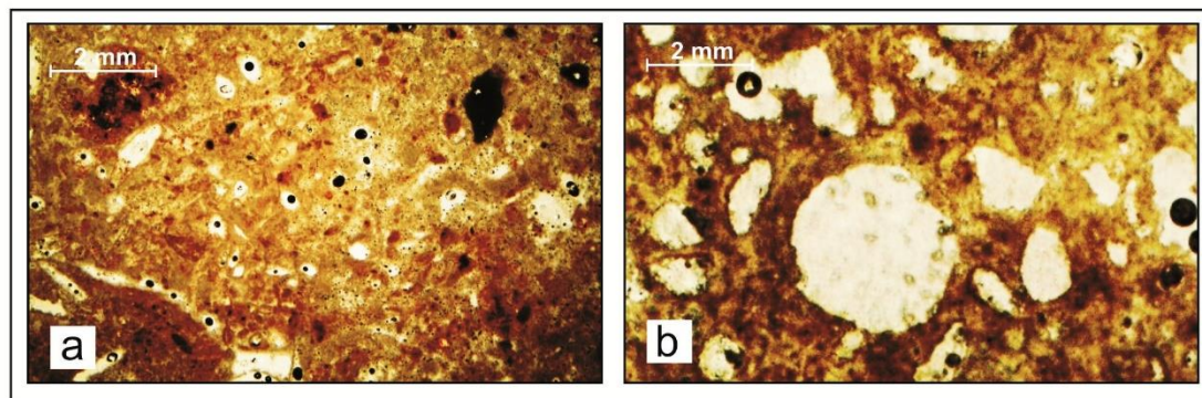
Fig. 7. Photomicrographs showing mostly mud-supported wackestone-packstone texture with common micrite-clasts (tiny brown pellets). The sediments in both microfacies are belonging to the Qaltah Member, the middle member of the Shurfah Formation (Upper Paleocene), at the Wadi Marzuq section. Longitudinal and circular sections (white colors) of Dasycladacean and Codiacean green algae are quite evident at the lower levels (a). Indistinguishable shell fragments (white colors) with micrite envelopes, micrite-clasts (brown colors) and scarce grains of green algae (white tiny disks) are major contributors to the sediments at the upper levels (b).
