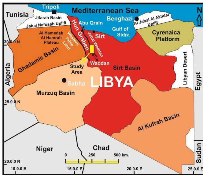
Fig. 1. Index map of Libya showing the major sedimentary basins of the country and the location of the study area, modified after Abdunaser and McCaffrey (2015).
