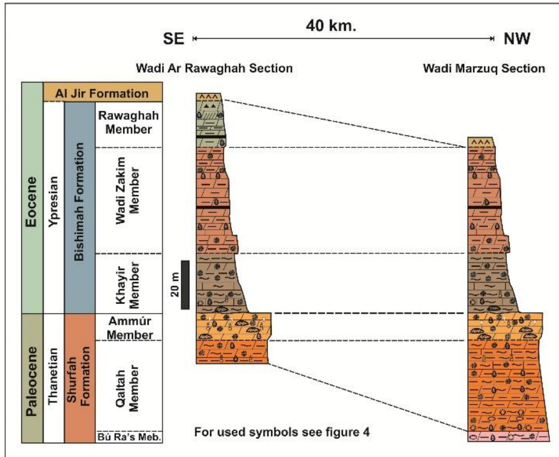
Fig. 5. Correlation chart showing the measured sections at Wadi ar Rawaghah and Wadi Marzuq. The correlation is based on all documented stratigraphical criteria.
