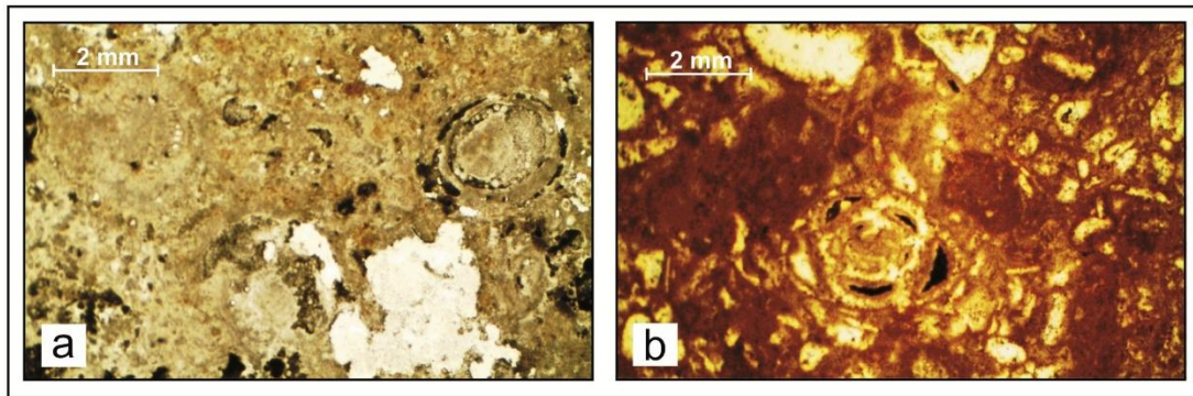
Fig. 11. Photomicrographs showing limestone with mud-supported wackestone-packstone texture. Both microfacies are belonging to the Rawaghah Member, the upper member of the Bishimah Formation (Lower Eocene), at Wadi ar Rawaghah section. Large-sized and globular forms of Alveolina sp. (right & left sides) (a) and large-sized Quinqueloculina sp.2 (at the middle) with scattered shell fragments of pelecypods (yellowish color) (b) are representing the main bioclasts components.
