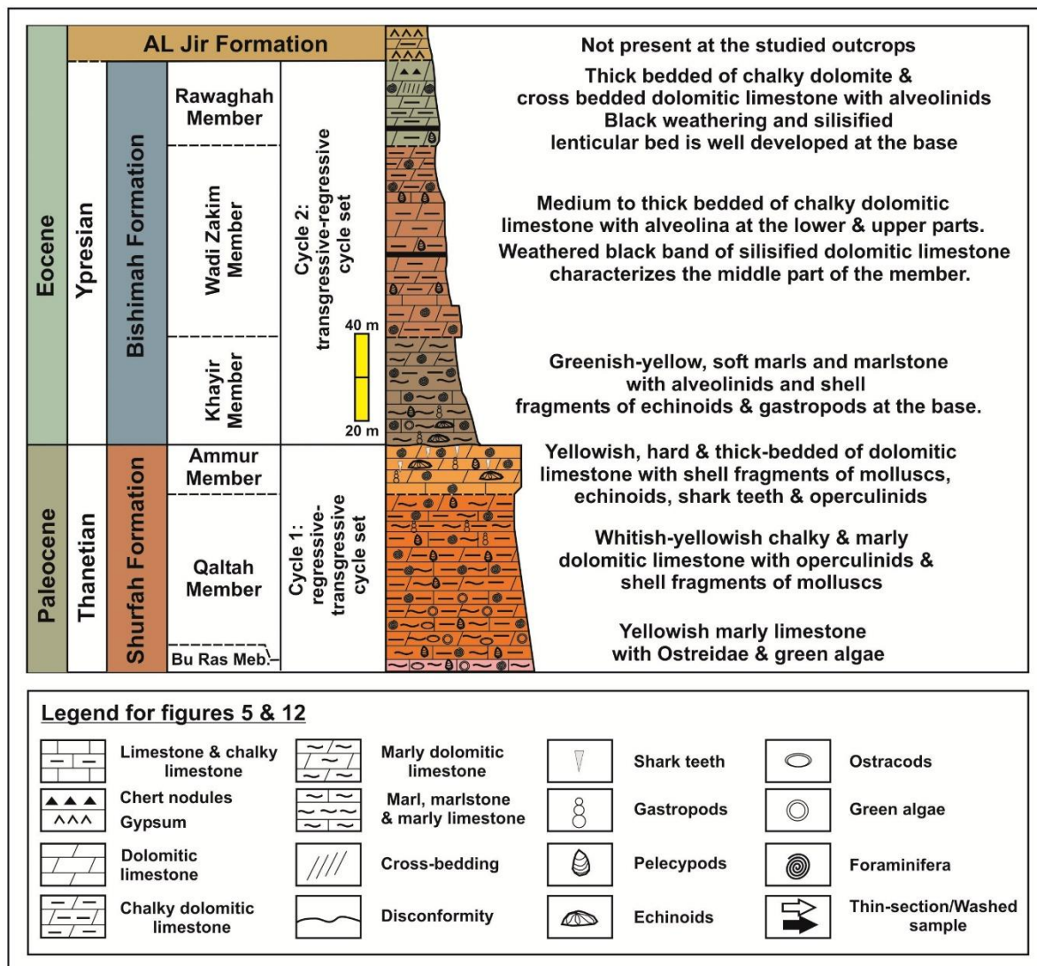
Fig. 4. Composite stratigraphic column of the study area showing the different characteristics of the Upper Paleocene/Lower Eocene stratigraphy in the study area and the main sedimentary cycles.
