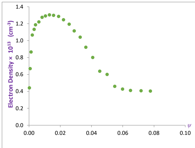
Fig. 8 The plasma electron density as a function of the flux parameter \psi .
