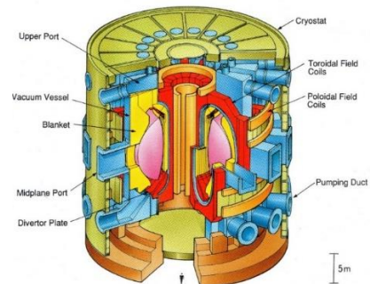
Fig. 2. International thermonuclear Experimental Reactor with Divertor Facilities, (curtesy of ITER Group).
