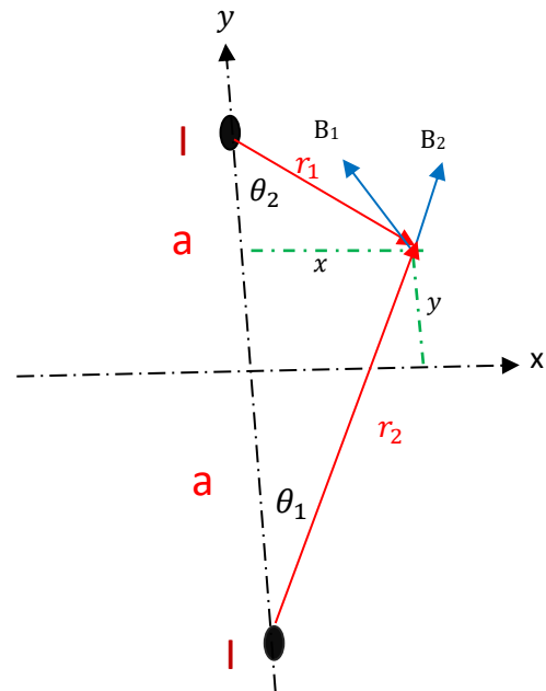
Fig. 4. Layout geometry used to show the structure of the magnetic field components in (x, y) plane.
