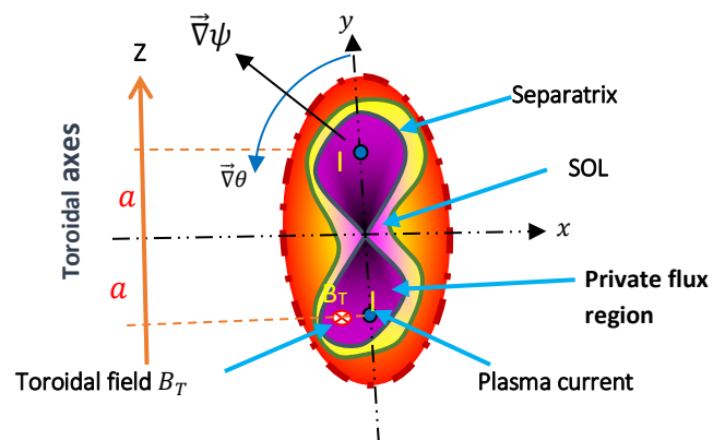
Fig. 1. Plasma cross-section with magnetic divertor configuration including Scarp Off Layer (SOL).
