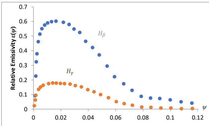
Fig. 6. The relative plasma emissivity \epsilon(\psi) calculated for the H_\beta and H_\gamma hydrogen lines.
