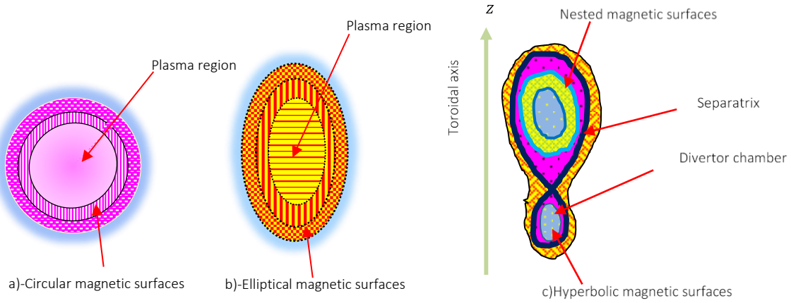
Fig. 3. Different shapes of magnetic surface configuration.
