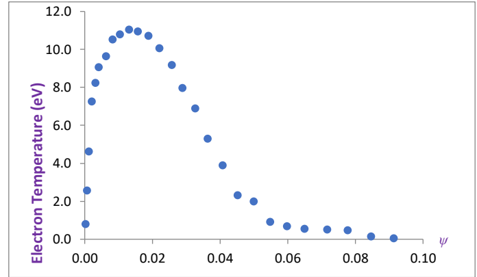
Fig. 7. The plasma electron temperature as function of the flux parameter \psi .
