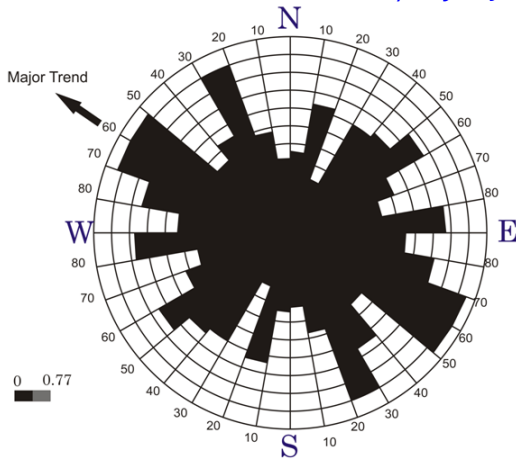
Fig. 8. Rose diagram representing the direction of 295 joints measured at Wadi Zazah, Al Jabal Al Akhdar, NE Libya.
