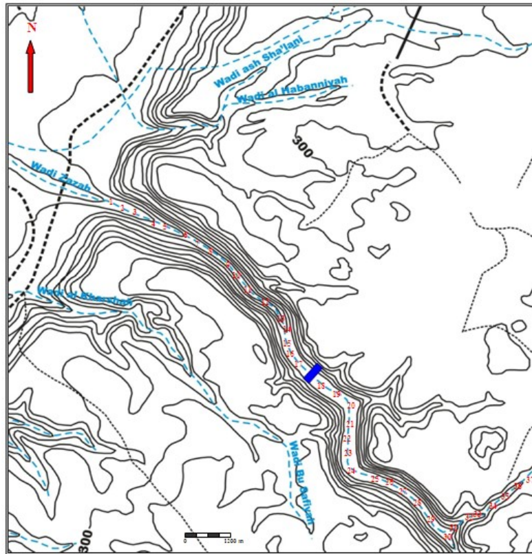
Fig. 4. Topographic map of Wadi Zazah showing the location of stations for measuring the altitude and direction of the recognized terrace fragments. 1-37 measuring stations; ■ Wadi Zazah Dam.
