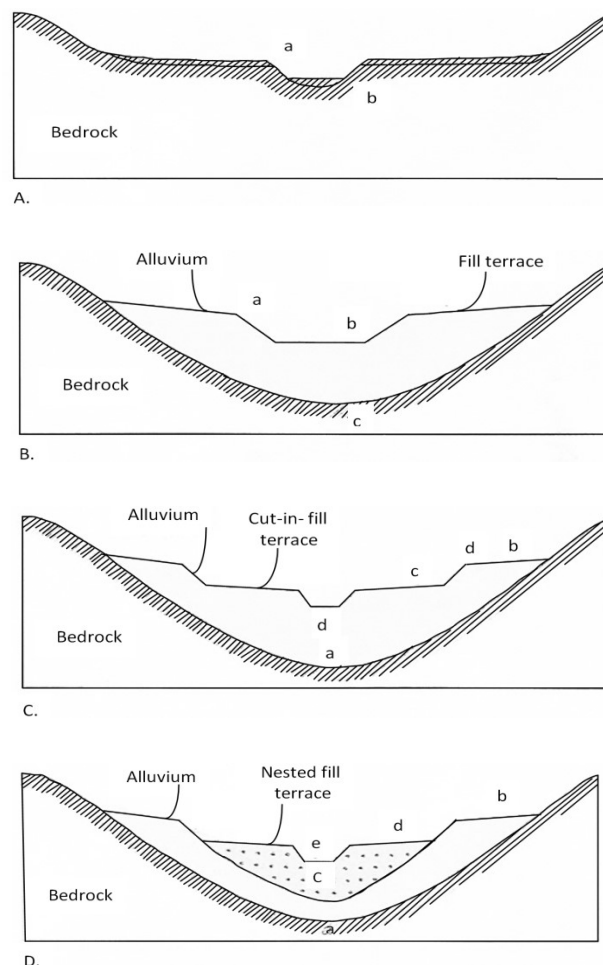
Fig. 3. Types of stream terraces: (A) bedrock (cut) terrace, (B) fill terrace, (C) cut-in-fill terrace, (D) nested fill terrace.
