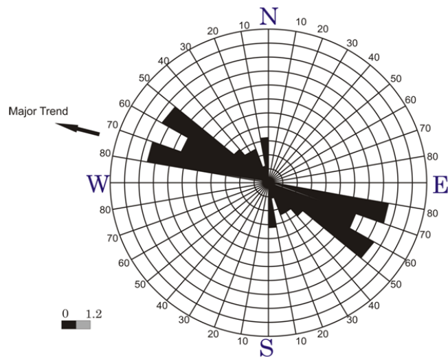
Fig. 7. Rose diagram representing the direction of (37) terrace fragments at Wadi Zazah, Al Jabal Al Akhdar, NE Libya.
