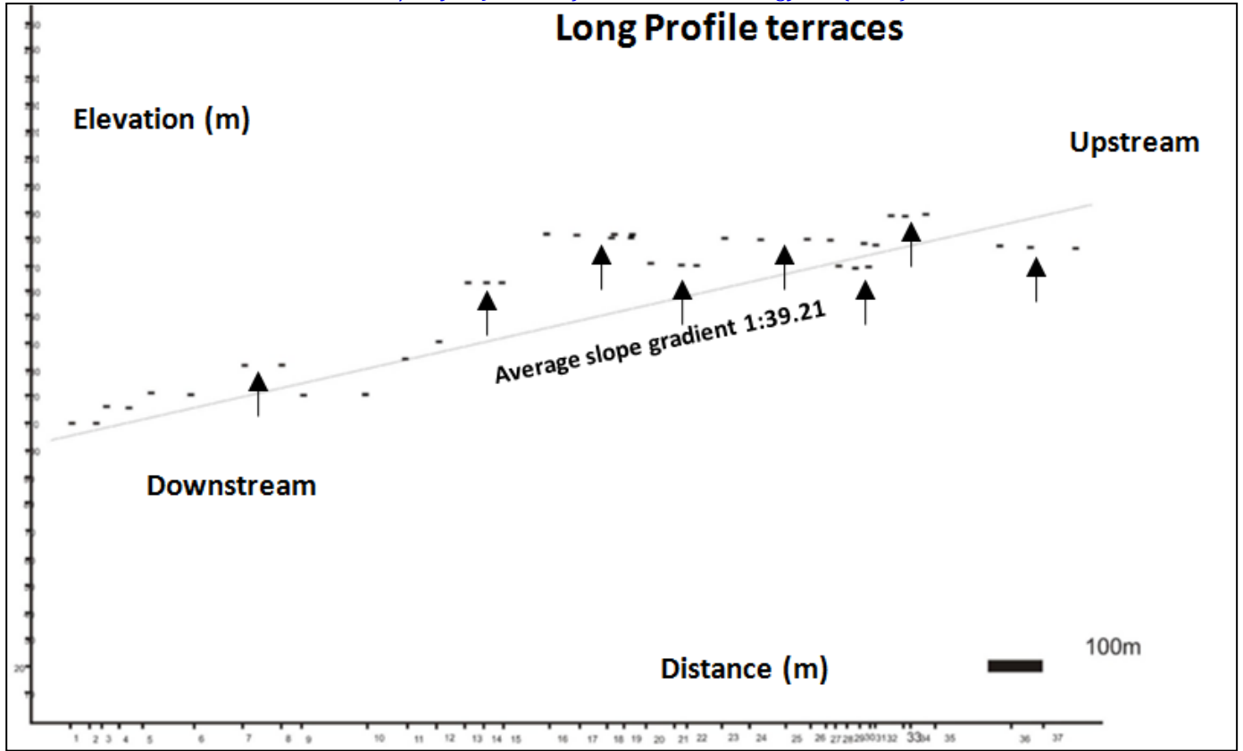
Fig. 6. Reconstructed long valley profile of the terrace fragments measured at Wadi Zazah, Al Jabal Al Akdar, NE Libya.
