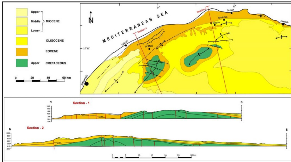
Fig. 2. Geological map and cross sections of northern Cyrenaica (from: El Hawat & Shelmani, 1993).
