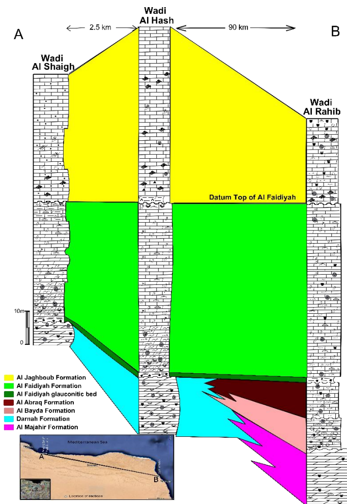
Fig. 14. Stratigraphic correlation shows the lateral variation on lithotypes of the Pre-transgressive glauconitic bed.
