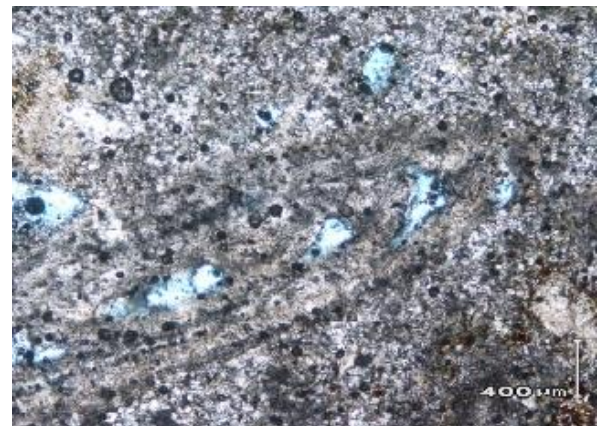
Fig. 8. Nummulites gizehensis in dolomitic grainstone from the Darnah Formation at Wadi Al Hash.
