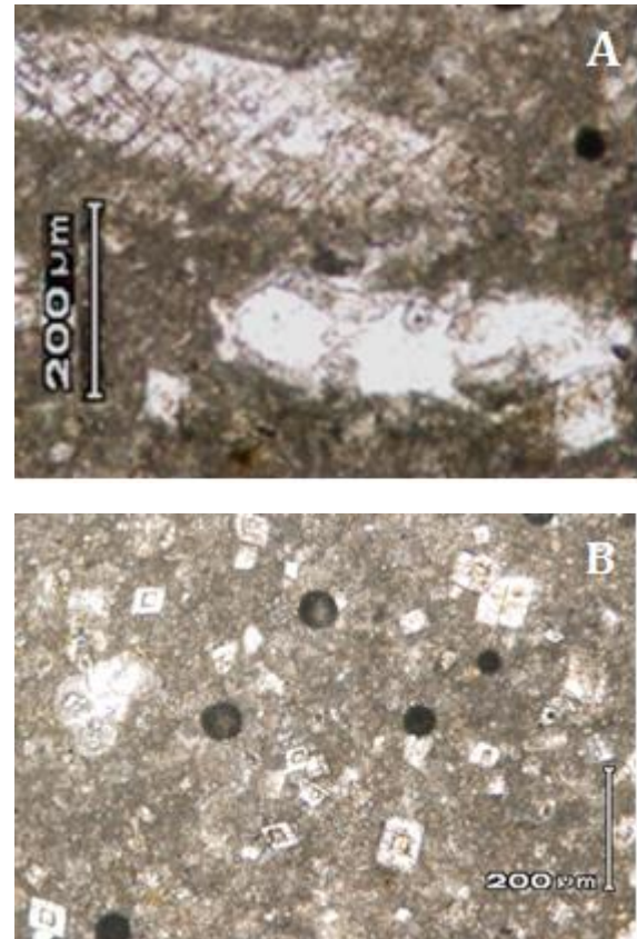
Fig. 5. A) Inoceramus prisms and Globotruncana sp.; B) Heterohelix globulosa , Al Majahir Formation at Wadi al Rahib. (Note: scattered euhedral dolomite crystals are commonly zoned with clear rim and the inner part (core) is more cloudy).
