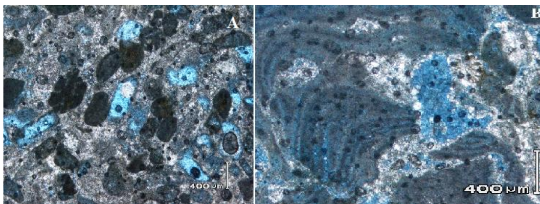
Fig. 12. Photomicrographs of Al Jaghboub limestone; A) showing scattered ellipsoidal grains of an algae of peloids limestone textures; B) destructive fabric of red algae by dolomite crystals, the spar filled holes within the skeleton at Wadi al Hash section.
