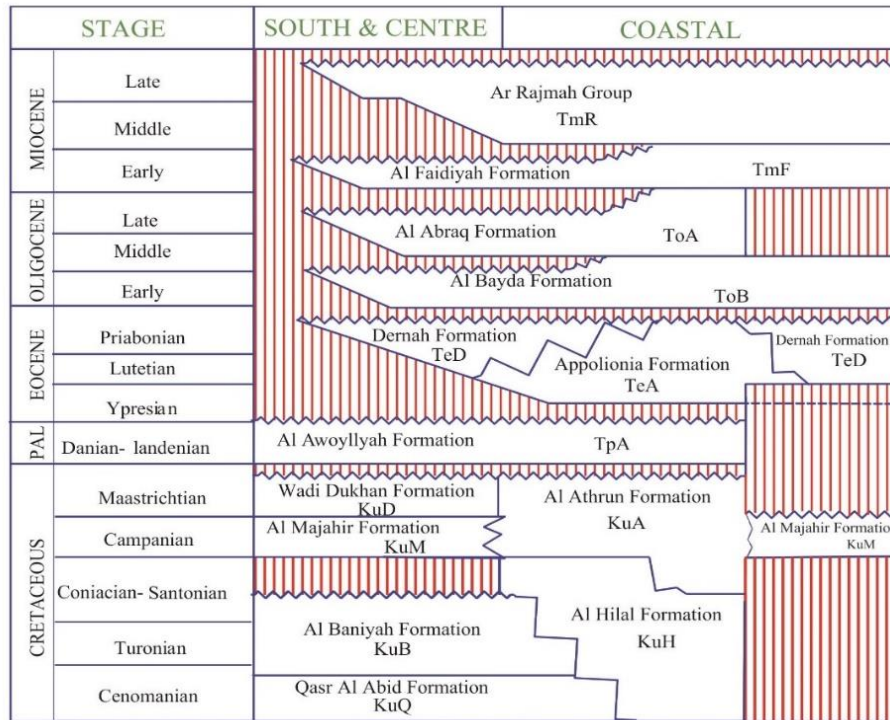
Fig. 3. Stratigraphical chart of northern Cyrenaica (Modified after El Hawat and Shelmani, 1993).
