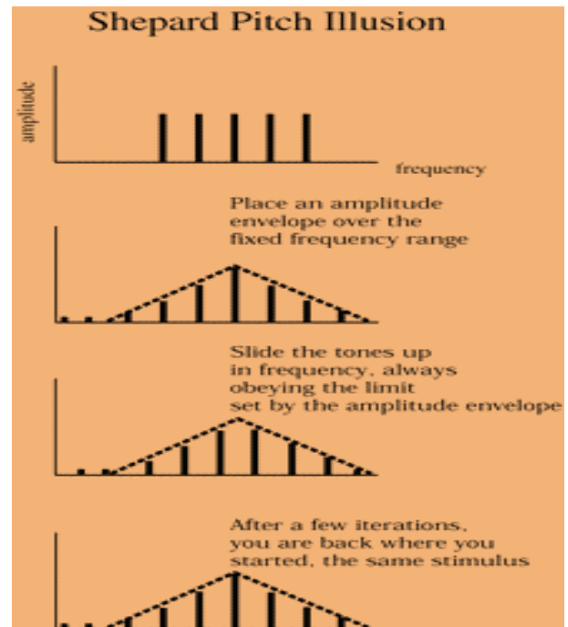
Fig. 25. The Shepard pitch Fourier spectra (Heeger, 2006).
