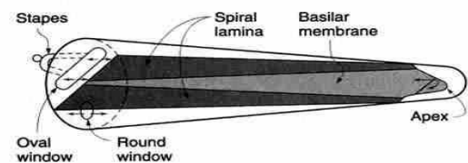
Fig. 11: The basilar membrane is not homogeneous (Heeger, 2006).
