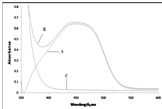
Fig. 1. Absorption spectra of 5 ppm SDz treated according to the recommended procedure Vs. reagent blank (A), distilled water (B), and blank solution measured Vs. distilled water
