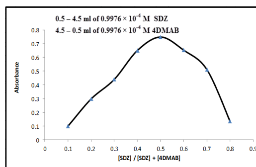
Fig. 5. (a) Continuous variations (Job) plot
