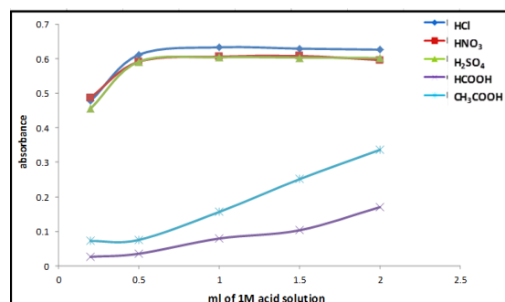
Fig. 2. Effect of 1M acid solutions on absorbance
