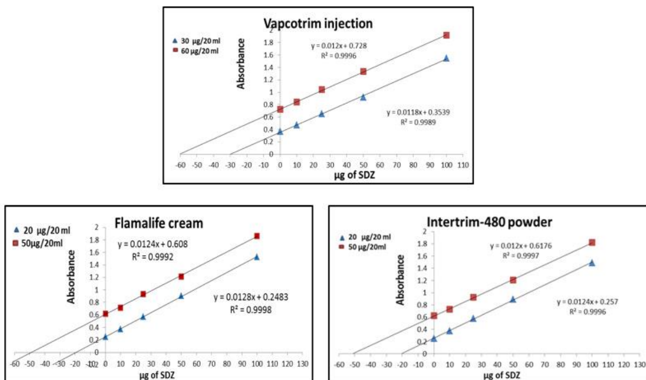
Fig. 6. Calibration graphs of standard additions method for the estimation of SDz in (a) injection, (b) powder, and (C) burn cream
