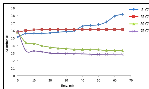
Fig. 3. Effect of temperature and time on absorbance
