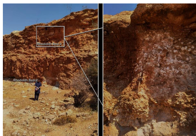
Fig. 9. The algal boundstone facies of Rhodoliths bearing bed - 3 at Farkash Quarry (FQ) section with closer view showing the rhodoliths (in white).
