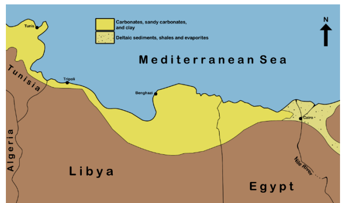
Fig. 4. Facies map showing the different sedimentary facies of the middle Miocene invaded sea deposits in North Africa (modified after Sherif, 1991).
