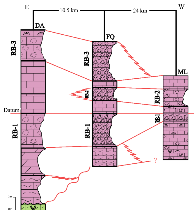
Fig. 14. Lithological correlation between the studied sections (Daryanah-Abyar (DA), Farkash Quarry (FQ) and Majdoub Lake (ML) sections). The top of the first Rhodoliths bearing bed -1 is used as datum.
