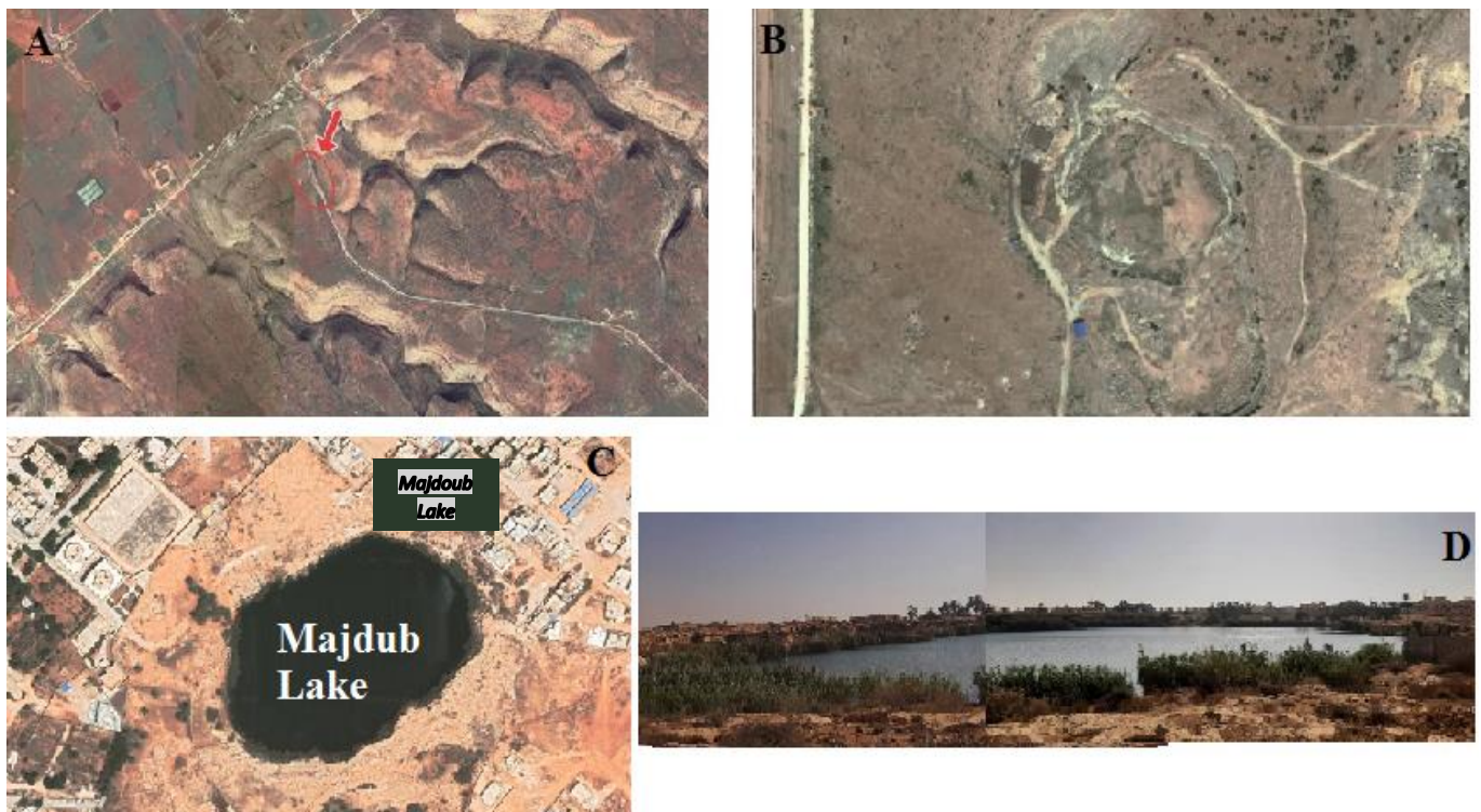
Fig. 2. Satellite images of A) Daryanah-Abyar (DA) roadcut (red arrow); B) Farkash Quarry (FQ); C) Majdoub Lake (ML). D) a general view of the Majdoub Lake (ML).
