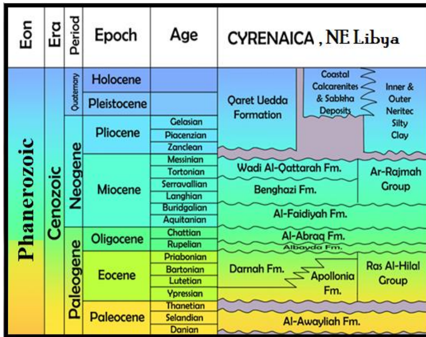
Fig. 3. Stratigraphic chart of northern Cyrenaica (after El Hawat and Abdulsamad, 2004).
