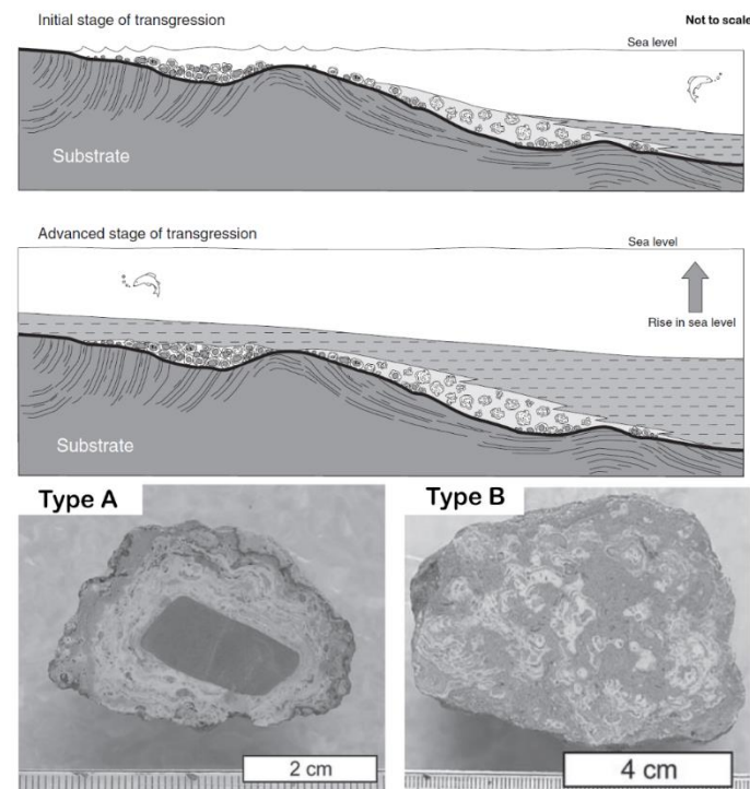
Fig. 15. Depositional model of the transgressive rhodolitic units. In the initial stage of transgression, Type-A of rhodolith form in shallow high-energy settings and are often localized in topographic depressions of the substrate. Type B units develop in calmer, possibly deeper waters and present a matrix-supported texture with rhodoliths showing a loose internal structure. In the advanced stage of transgression, basal fine-grained units are deposited directly above the rhodolitic accumulations. The result in succession rests above a major unconformity and is characterized by a deepening upwards trend. The size of Rhodoliths increases gradually by depth and distance from the shore line (After Nalin et al., 2007).
