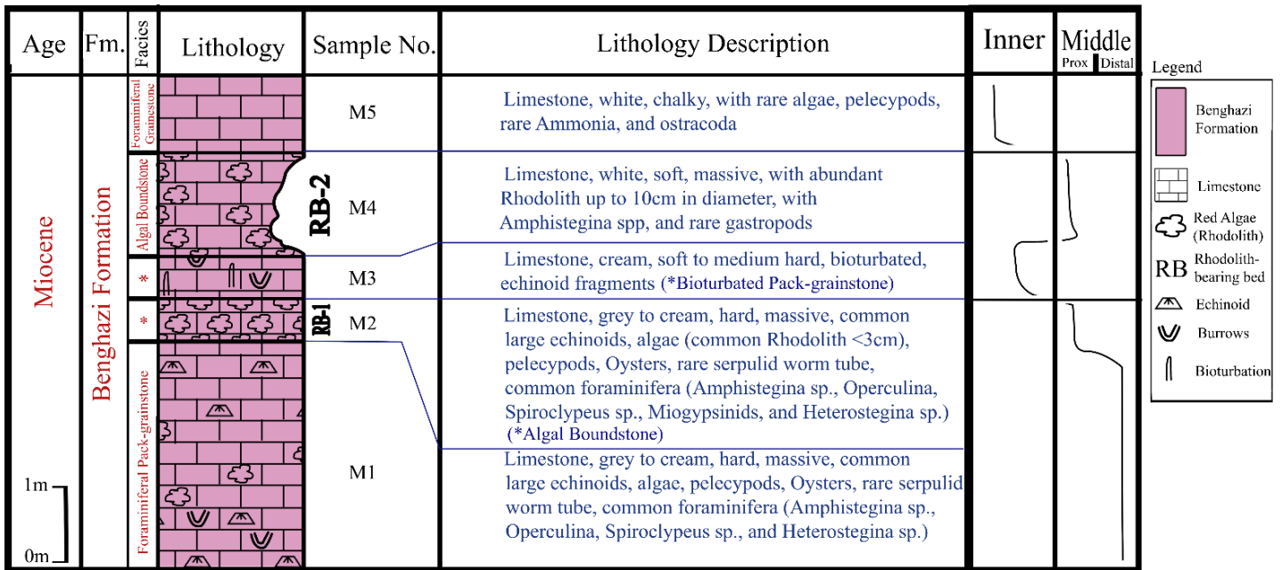
Fig. 12. Lithological column of Majdoub Lake (ML) section showing the lithological facies against the depositional environment curve.
