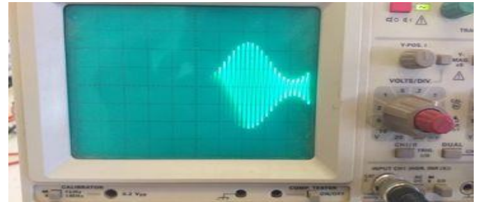
Fig. 30. The output amplitude modulated wave at point (b) after connecting the LC resonant circuit in Fig. 21 ( V_m = 6 V, V_c = 11 V).
