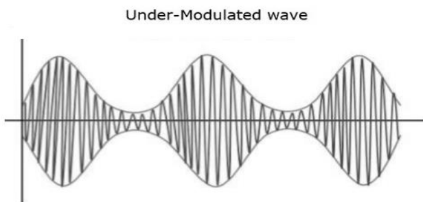
Fig. 3. The under-modulated wave.
