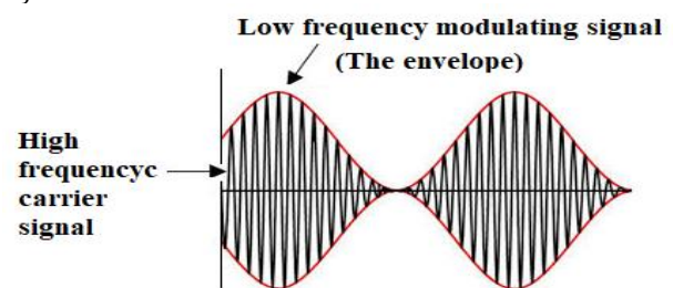
Fig. 1. AM signal in time domain.
