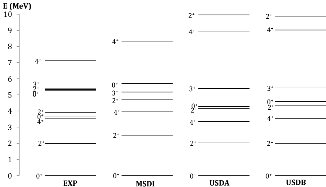
Fig. 1. Calculated energy levels for ^{18}\text{O}_{10} nucleus in comparison with experimental data (EXP) (Tilley et al. , 1995) and previous theoretical work (Hasan, 2018) denoted by USDA and USDB.
