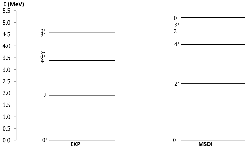
Fig. 2. Calculated energy levels (MSDI) and the experimental values (EXP) (Tilley et al., 1995) of ^{18}_{10}\text{Ne}_8 .
