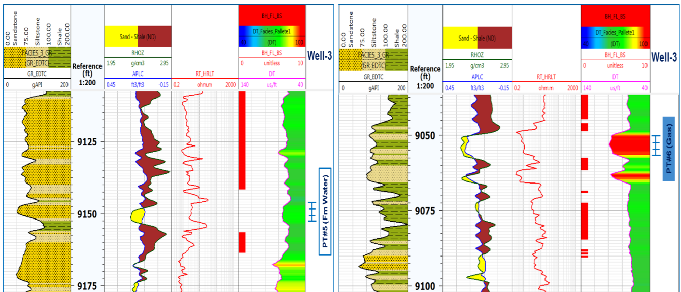
Fig. 9. (A) Production test near the top part of Lower Acacus reservoir shows a good fit between water interval in PT#5 and (B) Gas interval in PT#6 with DT_Facies_Palette1.
