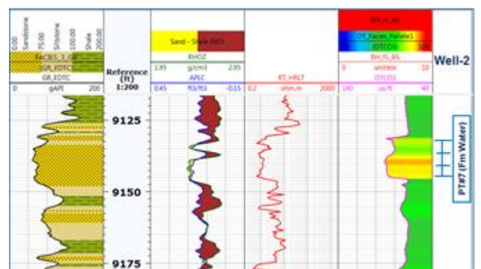
Fig. 8. (A) and (B) production test near the top part of Lower Accus reservoir shows a good fit between water intervals and DT_Facies_Palette.
