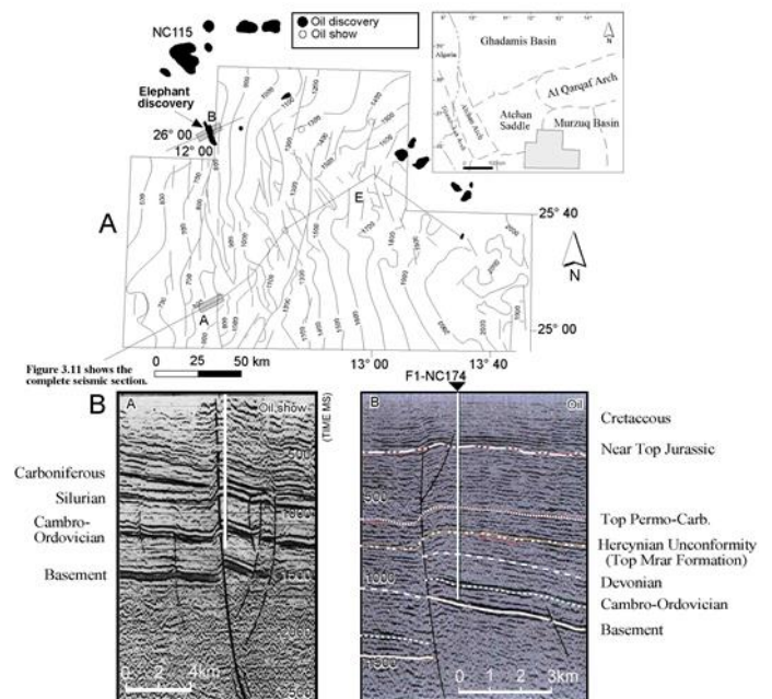
Fig. 7. A) TWT structural map (Middle Devonian unconformity), C.I.20 msec, showing N-S en-échelon fault blocks. The fault system is part of the 10° wrench zone. B) Seismic windows, the seismic sections showing flower structure in concession NC58 (window A) and reverse faulted anticline formed over a basement uplift (window B). Well F1-NC174 is a well in the giant Elephant field, while the other well is a dry hole in a smaller but well-defined closure to the south.
